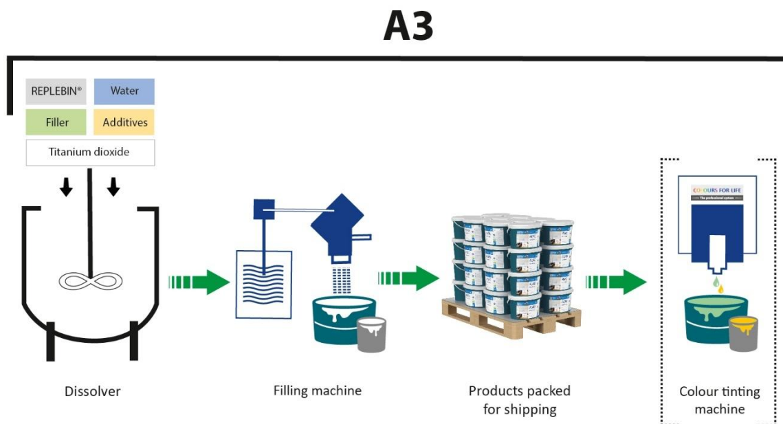
Figure 1 General Production Process
